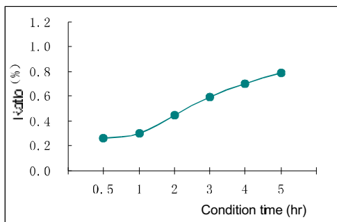
■ Water absorption at pressure cooker
