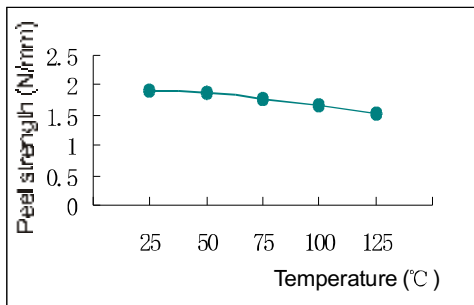
■ Peel strength
