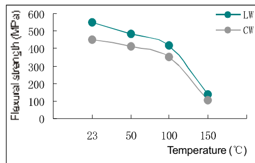
■ Flexural strength
