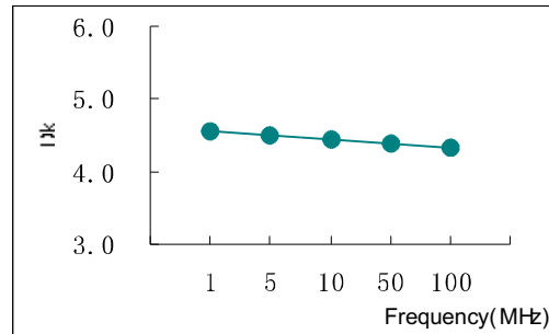
■ Dielectric constant
